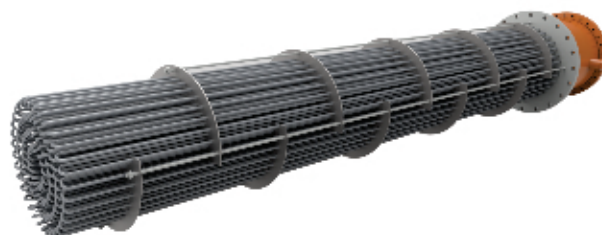
Segmental Baffle Assembly.
